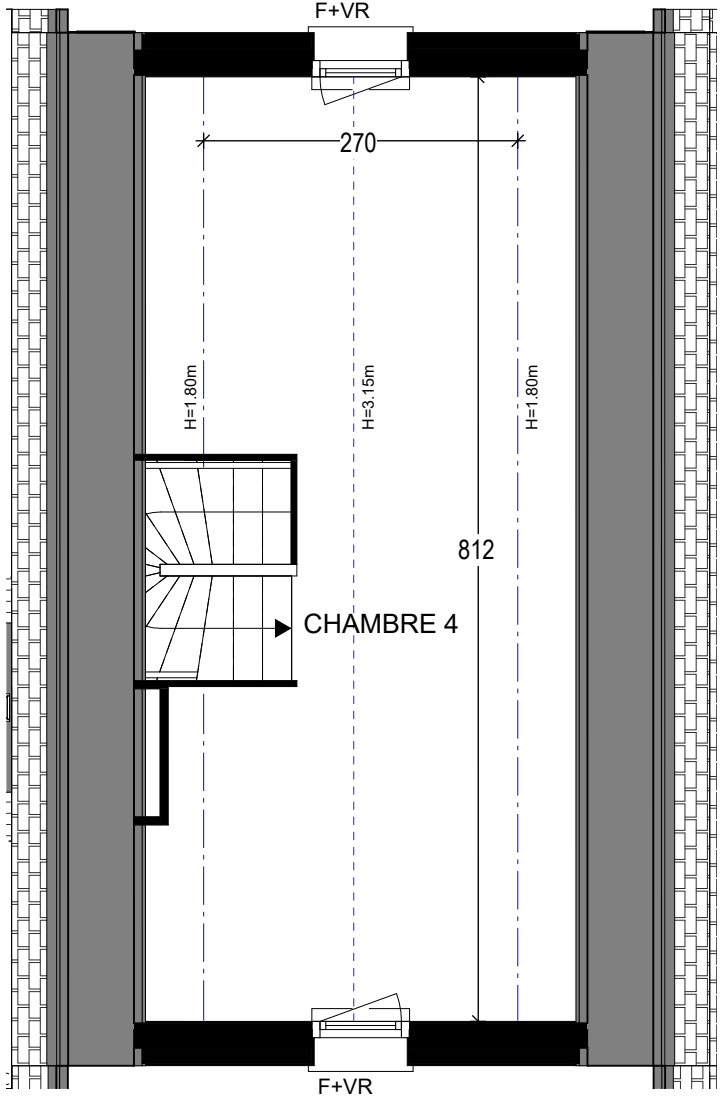
COMBLES
